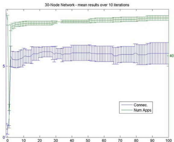
Figure 3. Reconstitution metrics for a 30-node network. The horizontal axis represents time steps (arbitrary units) after a fault at time 0. The vertical axis shows the algebraic connectivity (blue, scale on left) and number of services operational (green, scale on right). The vertical bars represent the standard deviation over 10 random networks.
